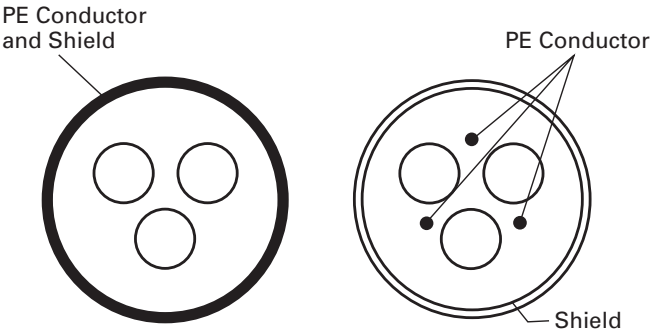
Figure 31. Cable description
