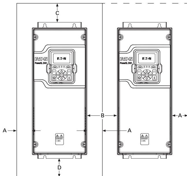
Figure 16. Mounting space
