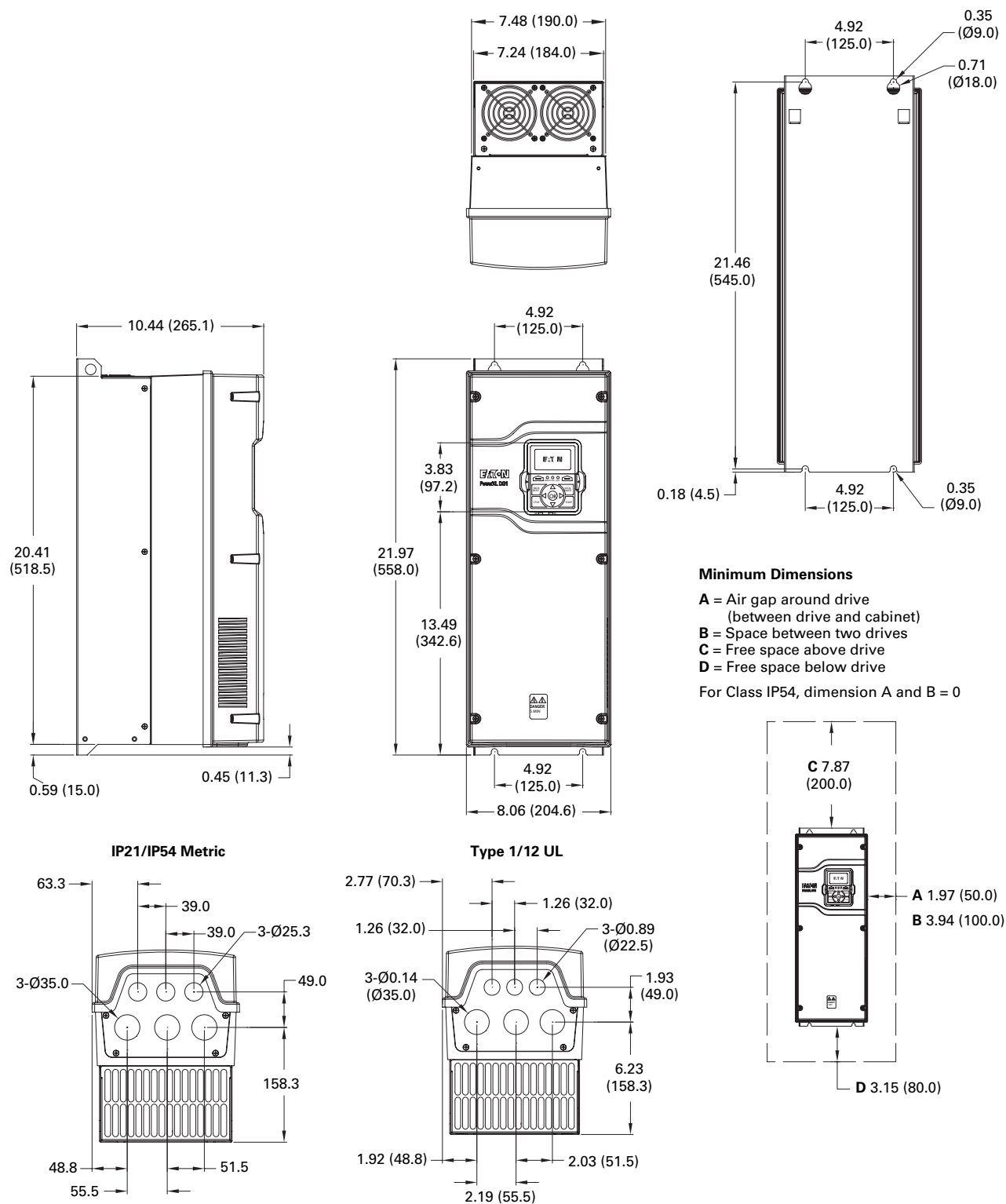
Figure 39. FR3 Dimension drawing
