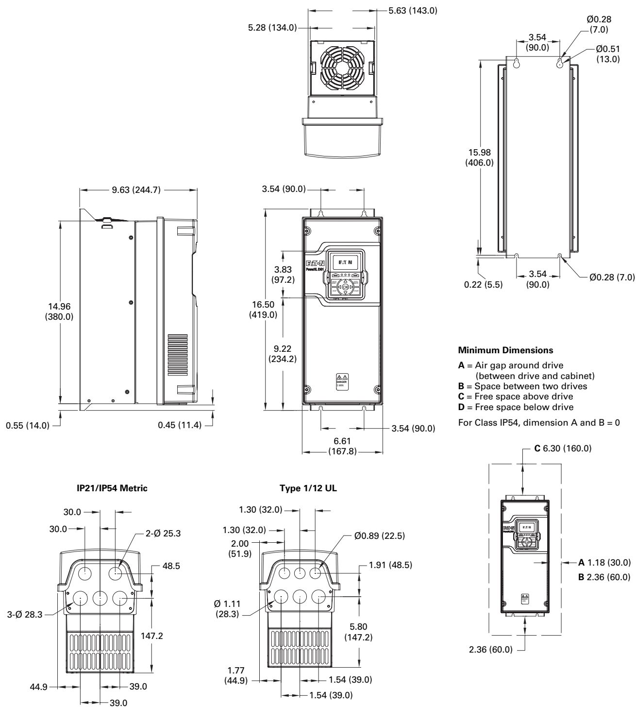
Figure 37. FR2 Dimension drawing
